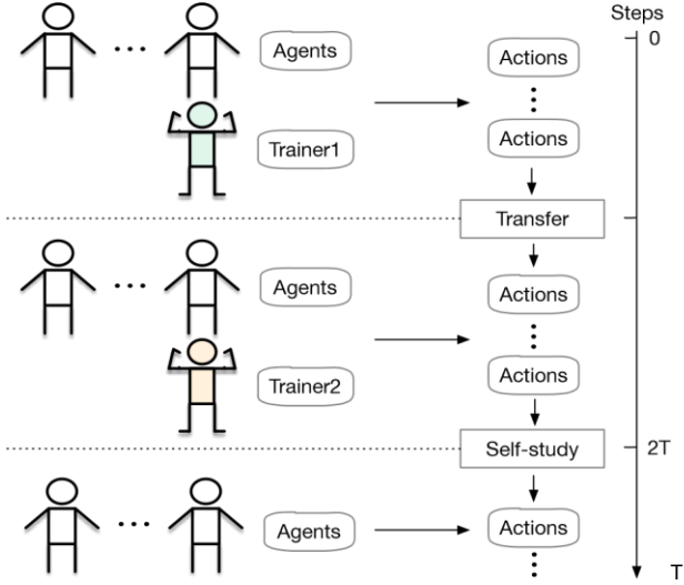
Fig. 4: General process of Hybrid Teaching strategy. One trainer gives advice firstly; then, another trainer gives advice. Finally, agents explore and learn by themselves.
