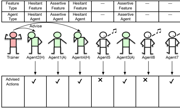
Fig. 3: General process of trainer guiding agents. Our framework firstly identifies assertive agents (labeled by ‘A’) and hesitant agents (labeled by ‘H’). Then, the trainer offers advice to hesitant agents.
