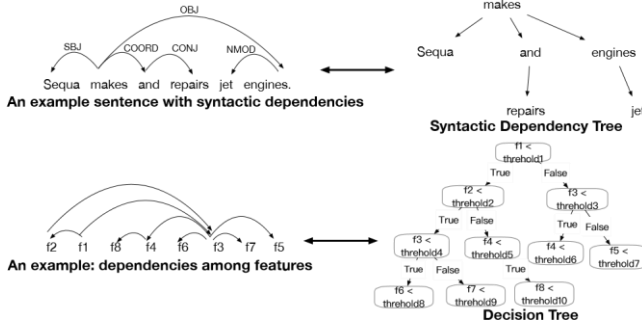
Fig. 5: In NLP, syntax dependencies and syntactic dependency tree. In our framework, dependencies among features and the decision tree.
