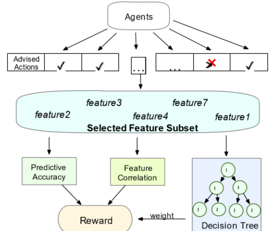
Fig. 7: General process of measuring reward with feature importance in the decision tree.
