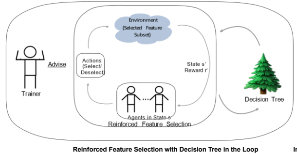
Fig. 1: Interactive reinforced feature selection via interaction with external trainers and downstream tasks (decision tree).
