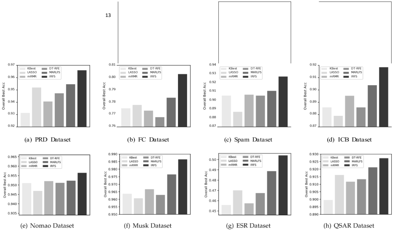
Fig. 9: Overall Best Acc of different feature selection algorithms.
